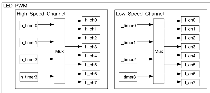
Figure 14-1. LED_PWM Architecture
